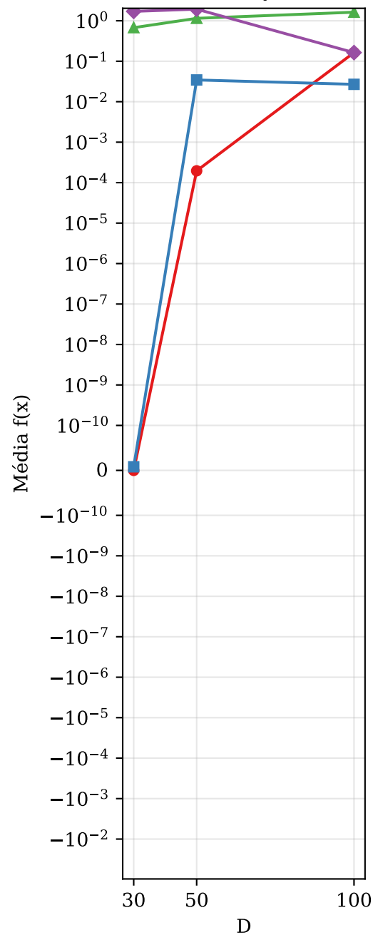
Ackley
