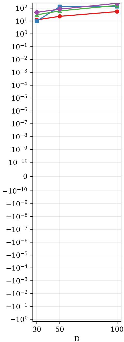
Rastrigin
